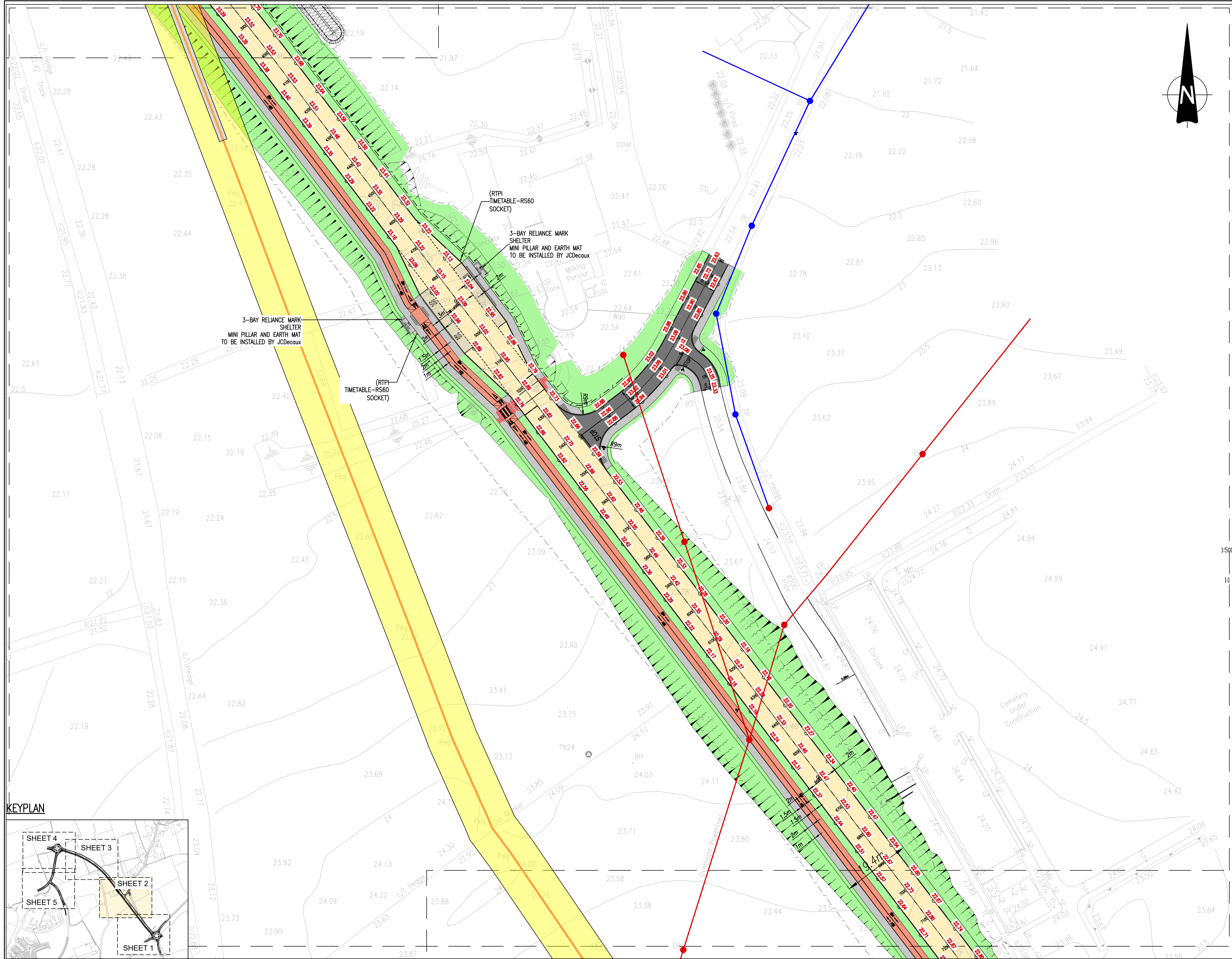
PLAN VIEW - PROPOSED ROADS LAYOUT AND LEVELS - SHEET 2 OF 5 SCALE 1:500 @A1
